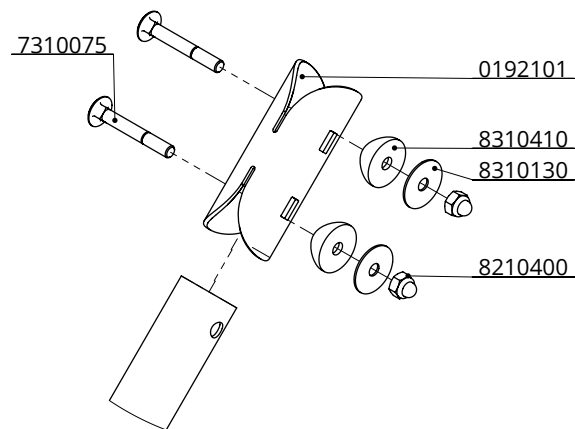
detail P (1 : 4)
