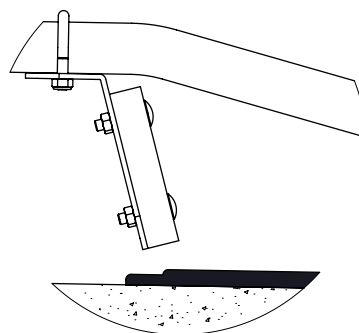
detail B (1 : 5)
