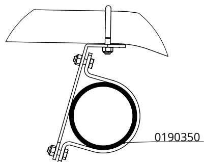
detail A (1 : 5)
