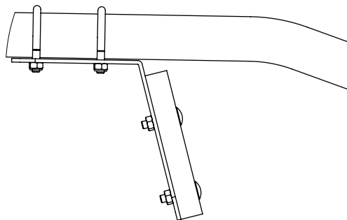
detail A (1 : 5)
